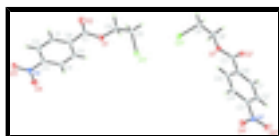
Fig. 1. eA view of the title compound with the atomic numbering scheme. Displacement ellipsoids were drawn at the 50% probability level.
